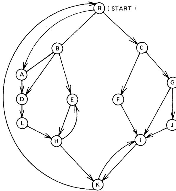
Fig. 1. A flowgraph
